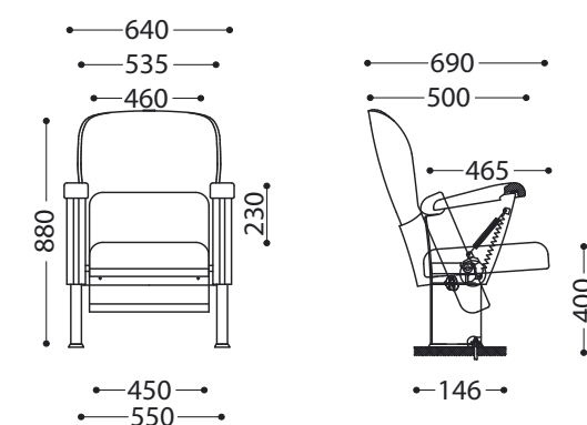
armchair Oscar W measurements in mm
