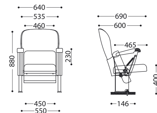
armchair Oscar measurements in mm
